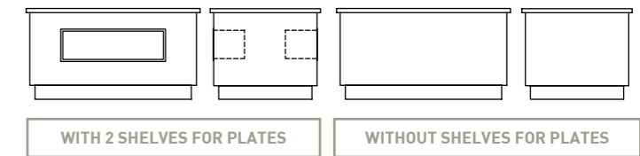
6GN module with 2 plates shelves and 2 shafts on the countertop, one for the embedment of 1 Drop-in well 2GN, and the other for 1 Drop-in well 3GN, model BDP11-6G/32
