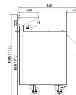
Optional counter kit, model KEB-160
