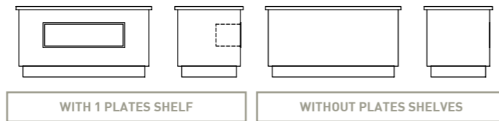
Module without plates shelves with shaft for 5GN, model BD8-5G/5
