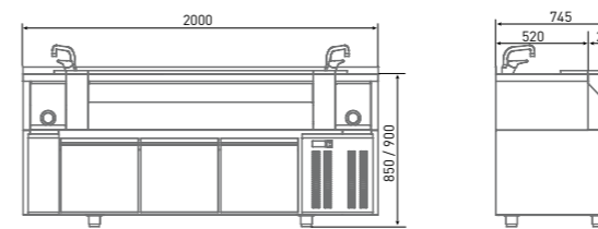
Model MBCR-200 + optional wells kit KCB-200
